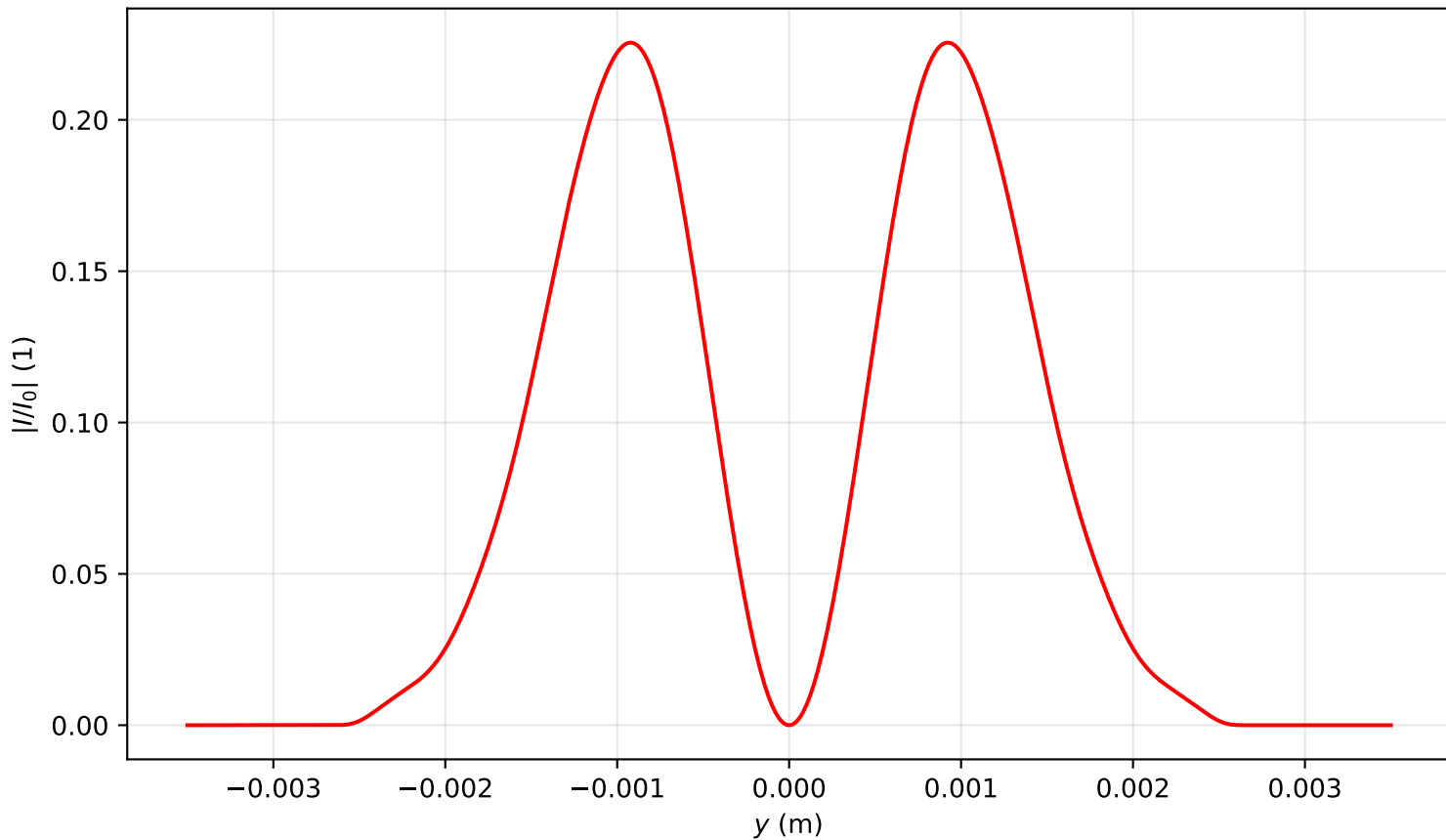
Intensity profile I(x=0, y, z=3.264)/I_0 , P_{in}=0.5P_{cr} , artificial time
